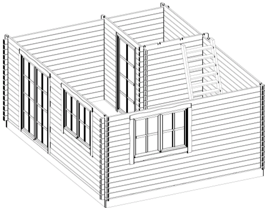
PERSPECTIVE RDC
